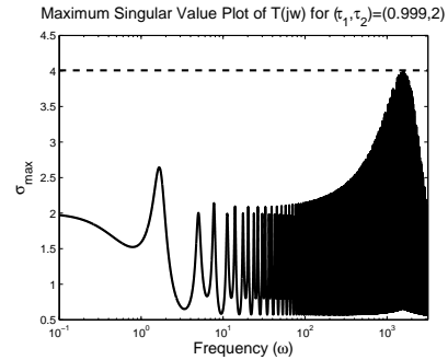
Fig. 5. The maximum singular value plot of T (16): \|T(j\omega, \tau)\|_\infty < \|T_a(j\omega, \tau)\|_\infty case.
