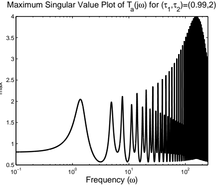
Fig. 3. The maximum singular value plot of T_a(j\omega) for (\tau_1, \tau_2) = (0.99, 2) as a function of \omega .
