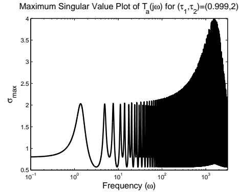
Fig. 4. The maximum singular value plot of T_a(j\omega) for (\tau_1, \tau_2) = (0.999, 2) as a function of \omega .
