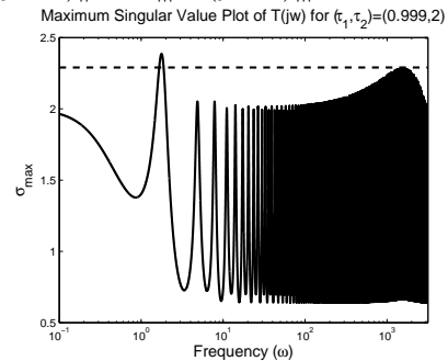
Fig. 6. The maximum singular value plot of T (26): \|T(j\omega, \tau)\|_\infty > \|T_a(j\omega, \tau)\|_\infty case.
