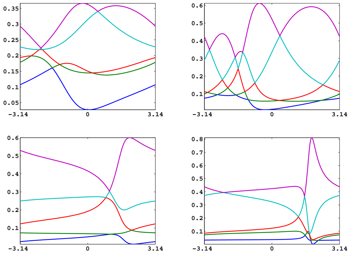
Figure 4: The weights of the of the quadrature formula with n = 5 points as a function of \theta \in [-\pi, \pi] where v = e^{i\theta} . The measure is d\mu(\theta) = (1 - \nu \cos(\theta))d\theta/(2\pi) . The poles are given by r(-1)^{1/5} . On the left for r = 0.72 and on the right for r = 0.9 . On top for \nu = 1 , at the bottom for \nu = -1 .
