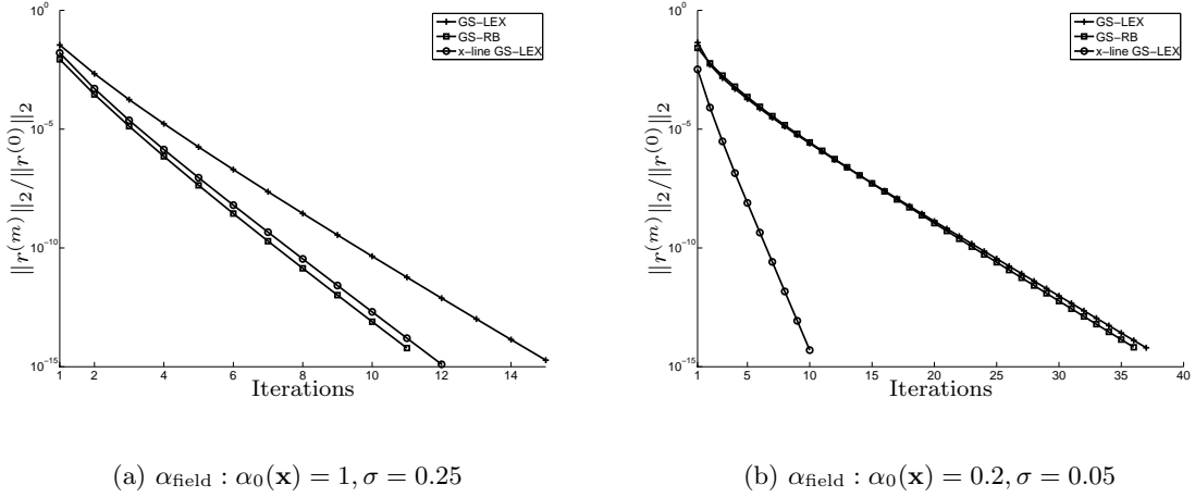
Figure 4: Residual norms for a V(2,1) multigrid cycle with pointwise lexicographic Gauss-Seidel (GS-LEX), pointwise red-black Gauss-Seidel (GS-RB) or lexicographic x -line Gauss-Seidel ( x -line GS-LEX) smoothing ( h = 2^{-4} , 2 nd order PC-basis, 4-term Karhunen-Loève expansion of \alpha_{\text{field}} with L_c = 1 ).
