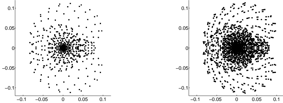
(b) \alpha \sim N(1.0, (0.1)^2) , 2^{\text{nd}} order PC-basis
