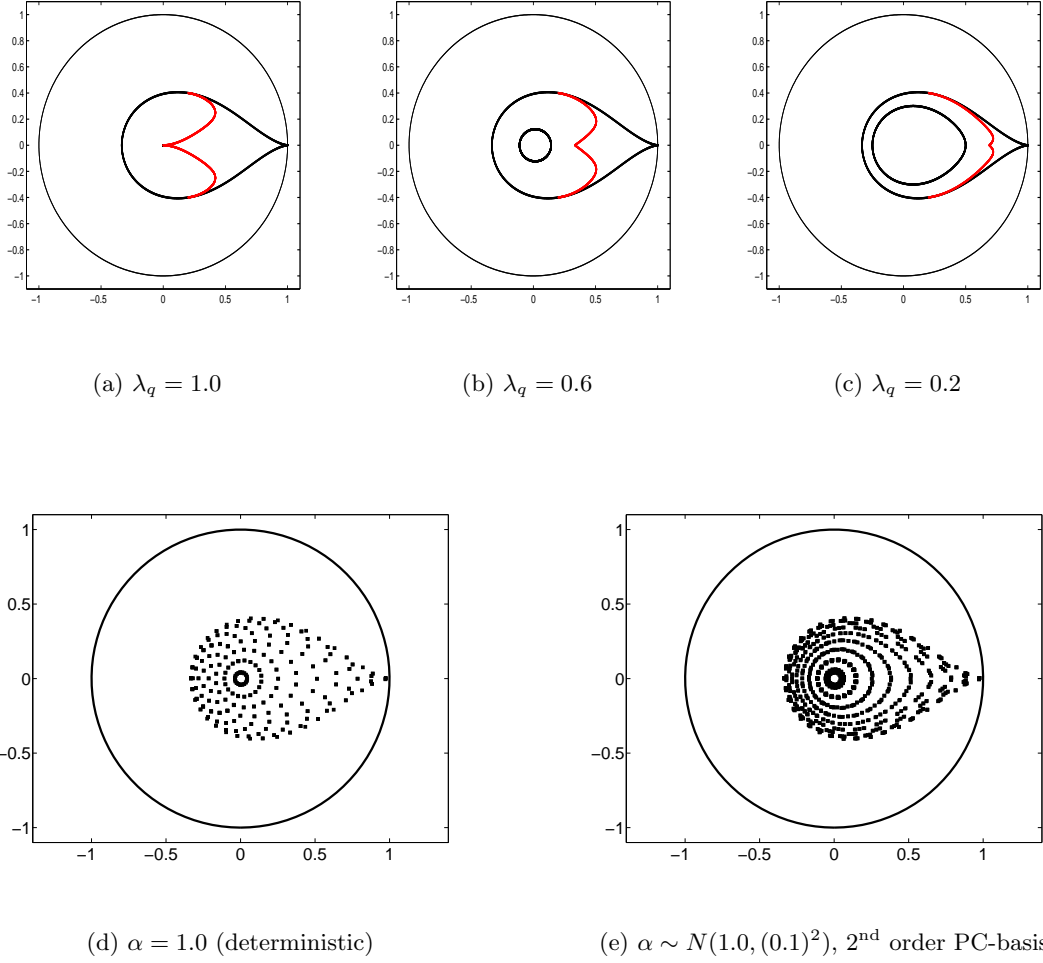
Figure 1: (a)–(c) Distribution of the eigenvalues for GS-LEX, for several values of \lambda_q : all the eigenvalues lie inside the unit circle, between the drop-shaped curve and the inner curve (which reduces to a point for \lambda_q = 1 ). The eigenvalues corresponding to the oscillatory modes lie at the left of the 3-shaped curve, those corresponding to the smooth modes at the right. (d)–(e) Eigenvalues for a deterministic and a simple stochastic problem (400 equidistant samples of (\theta_x, \theta_y) \in [\pi, \pi]^2 ).
