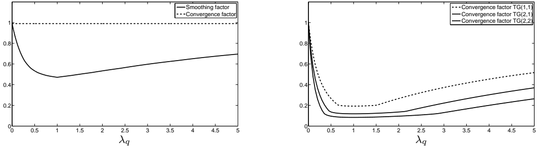
(a) Lexicographic Gauss-Seidel ( h = 2^{-5} )
