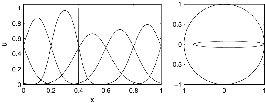
Figure 7: Some snapshots of the time-dependent reference solution u^*(t) of the convection-diffusion problem at t = 0, 0.1, 0.2, \dots, 0.5 . The initial condition is the scaled and shifted box function in the middle of the interval. The eigenvalues of the time-stepper are shown on the right.
