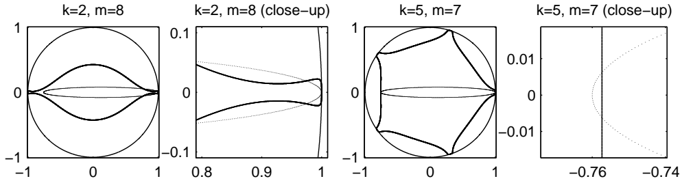
Figure 8: The eigenvalue spectrum of the convection-diffusion time-stepper and the boundaries of the stability regions \Omega_2(2, 8) and \Omega_2(5, 7) . Stability might get lost due to the imaginary eigenvalues near 1, or due to the real eigenvalues with smallest real part.
