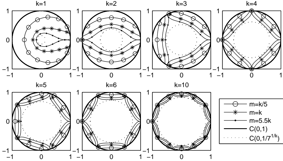
Figure 4: Some of the curves (17) for various values of k and m .
