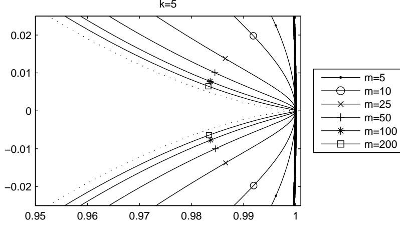
Figure 3: Tip formation as \mu increases. The thick line represents the unit circle. The thin lines are stability region boundaries for a fixed value of k (5) and various values of m (5, 10, 25, 50, 100 and 200). The dotted line is the limiting stability region boundary for \mu = 1 .
