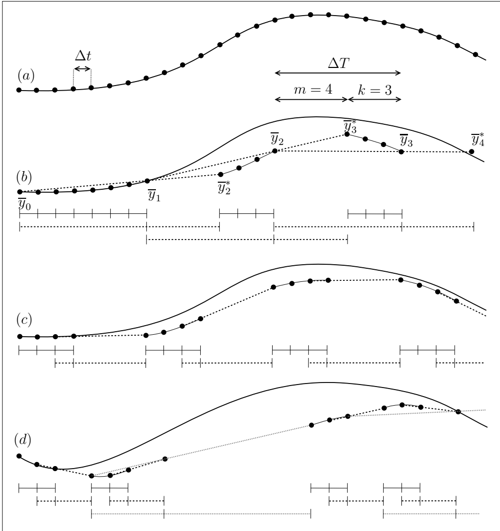
Figure 1: A schematic comparison of unaccelerated time-stepping (a), and accelerating the time-stepper using Algorithm 1 (b), PIM (c) or TPIM (d). All methods are based on linear extrapolation. In subfigures (b) and (c) we used k = 3 and m = 4 . In subfigure (d) we chose k = m = 2 and we added one extra level of recursion.
