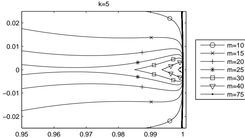
Figure 5: Detailed view of the stability regions \Omega_2(5, m) near 1 for various values of m . The thick line represents the unit circle. The thin lines are stability region boundaries for a fixed value of k = 5 and various values of m (10, 15, 20, 25, 30, 40, 75). No tip is formed but the stability region falls apart and the regions near 1 shrink fast for increasing values of m .
