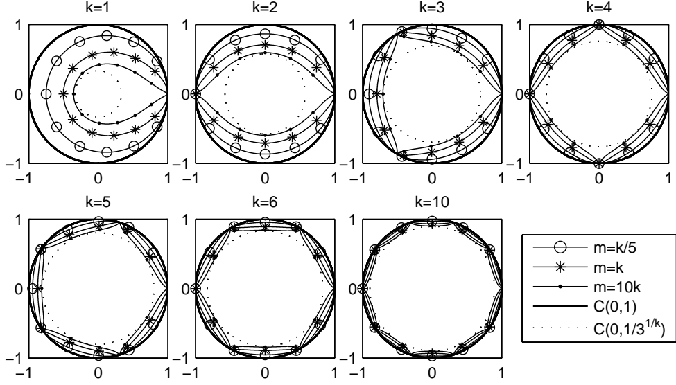
Figure 2: Some of the curves (4) for various values of k and m .
