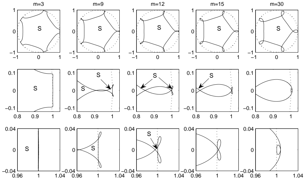
Figure 6: The curve P(e^{i\theta}, \rho(\theta), 5, \mu, 3) = 0 for several values of \mu . In each column, subsequent close-ups of the same curve are shown. The parts corresponding to the stability region (that are still visible) are indicated by the letter S. The dotted line is the unit circle.
