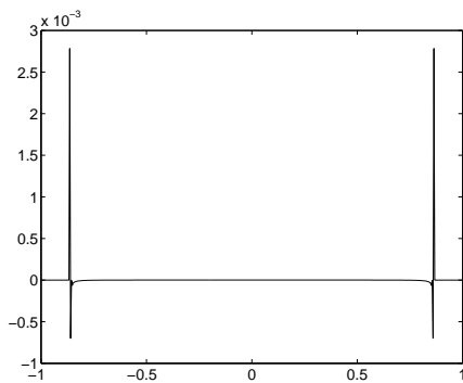
(b) Error of the computed solution of 4.1.1 with 500 equidistant discretization points
