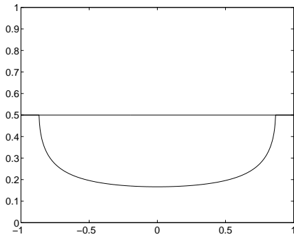
(a) Constraint \sigma and theoretical solution t\mu_t of 4.1.1
