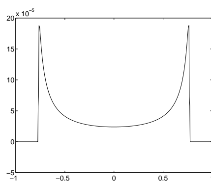
(e) Error of the computed solution of 4.1.2 with 500 equidistant discretization points
