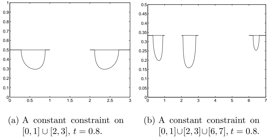
Figure 2. Numerical results for multiple intervals
