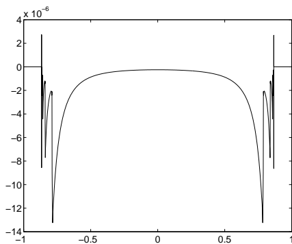
(c) Error of the computed solution of 4.1.1 after the refinement
