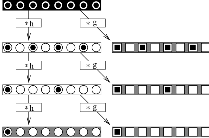
Figure 7: The redundant wavelet transform. The points with a black center represent coefficients that also appear in the decimated transform. To be consistent with this decimated transform, we should make sure that we only combine intermediate results from the original transform in our computation of coefficients “with a black center”.
