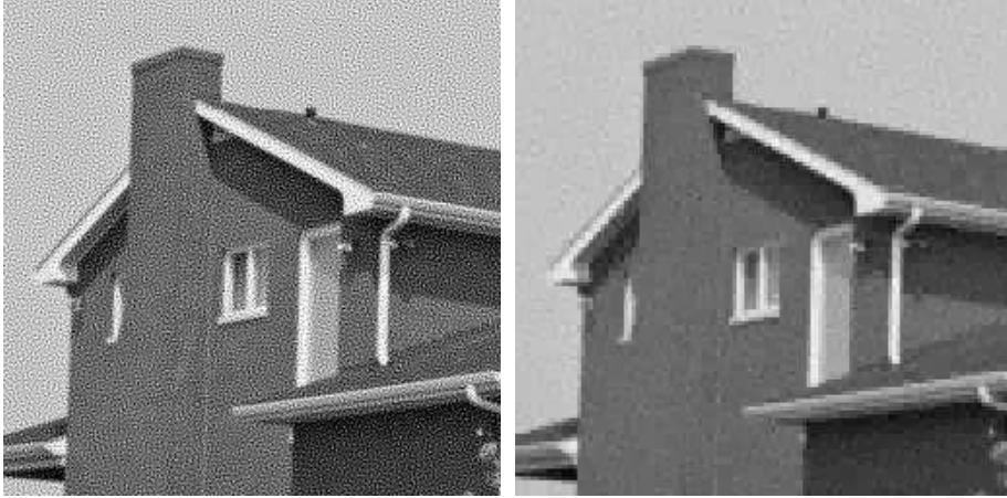
Figure 5: Left: an image with artificial, correlated noise. The noise is the result of a convolution of white noise with FIR highpass filter. Right: the result after level-dependent wavelet thresholding. We use Haar-wavelets.
