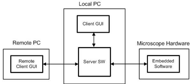
Fig. 1. Schematic diagram of the electron microscope software
