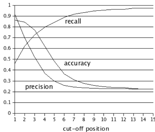
Figure 2: Average recall, precision and accuracy over 900 image-text pairs using different static cut-off values in the machine ranking.
